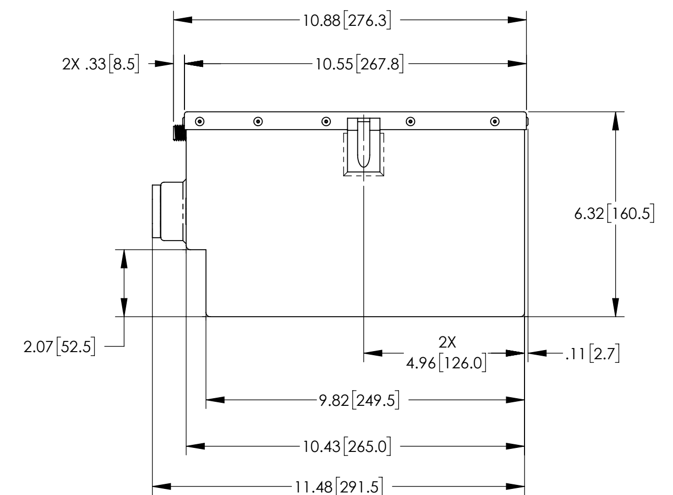
ENVELOPE DRAWING
