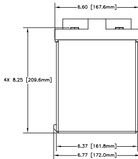
ENVELOPE DRAWING
